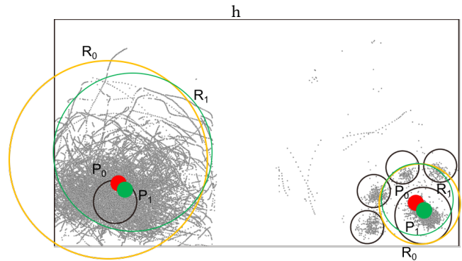
Figure 4: The selected area is represented by yellow and the original clustering center is indicated by a red dot; when choosing the parameter of confidence coefficient as 95%, the new clustering center is shown by a green dot and the new adjusted area is represented by a green zone.
